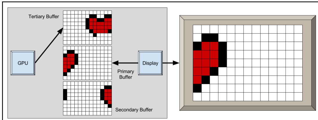
Figure 11.14 - Scenario 1 - Swapping all buffers after V-Blank
