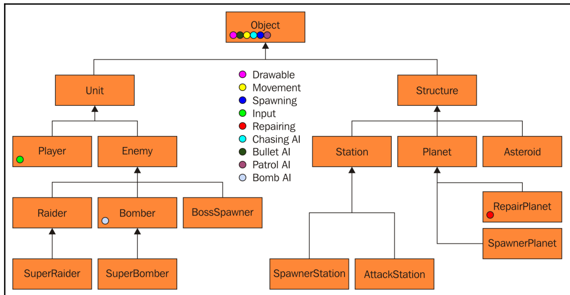
Figure 3 4 - After refactoring duplicate code to our base class (refer graphic bundle)
