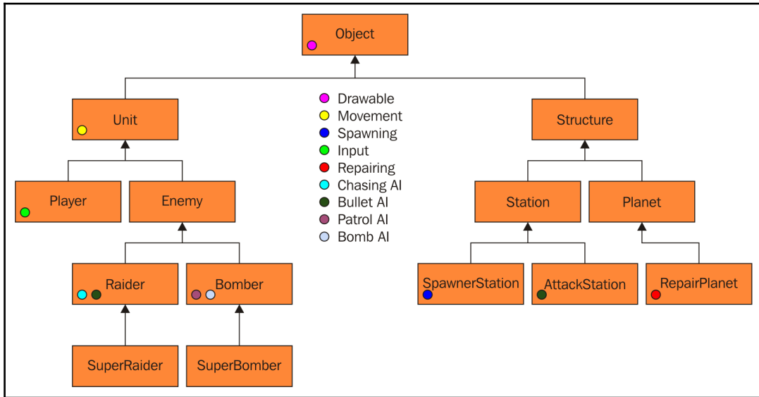
Figure 3.3 - After adding behavior to our objects (refer graphic bundle)
