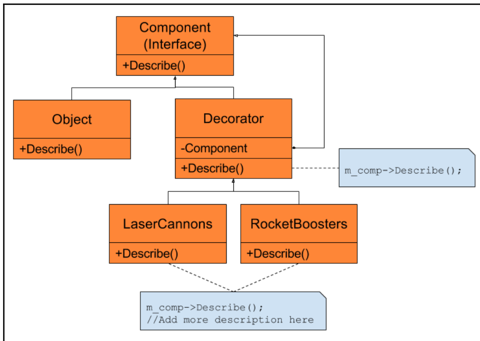
Figure 3.8 - The Decorator pattern using our Object
