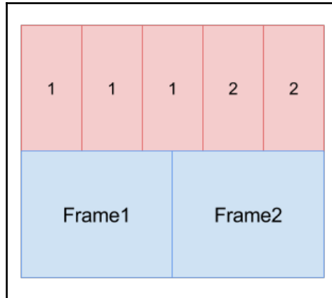
Figure 11.6 - Example of refresh rate and frames per second Out-Of-Sync
