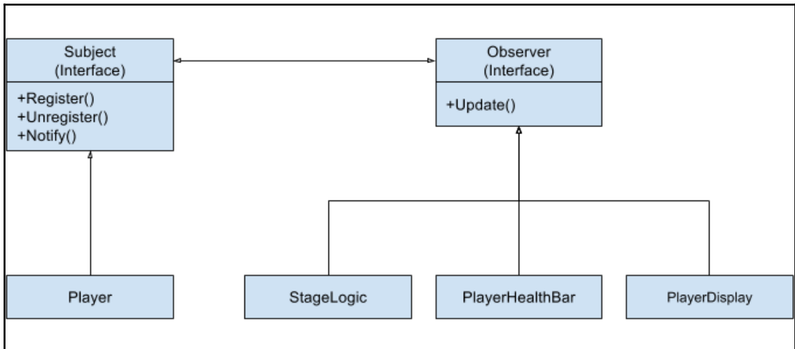
Figure 9 1 Interaction of Subjects and Observers
