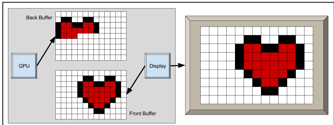
Figure 11.9 - Example of double buffering
