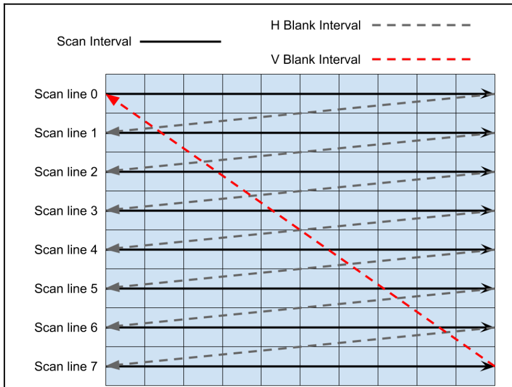
Figure 11.4-Showing the movement pattern of the electron gun including the Horizontal and Vertical Blank Intervals
