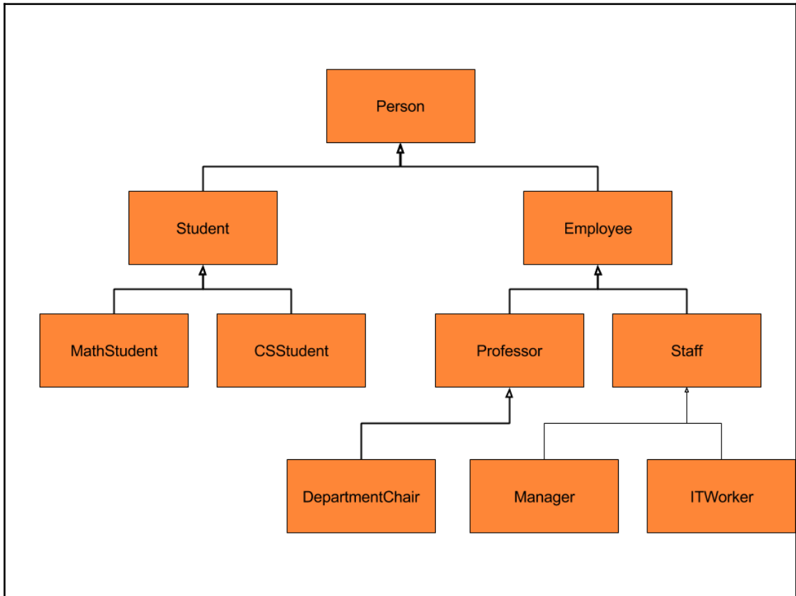
Figure 3.1 - A typical inheritance diagram when learning to program
