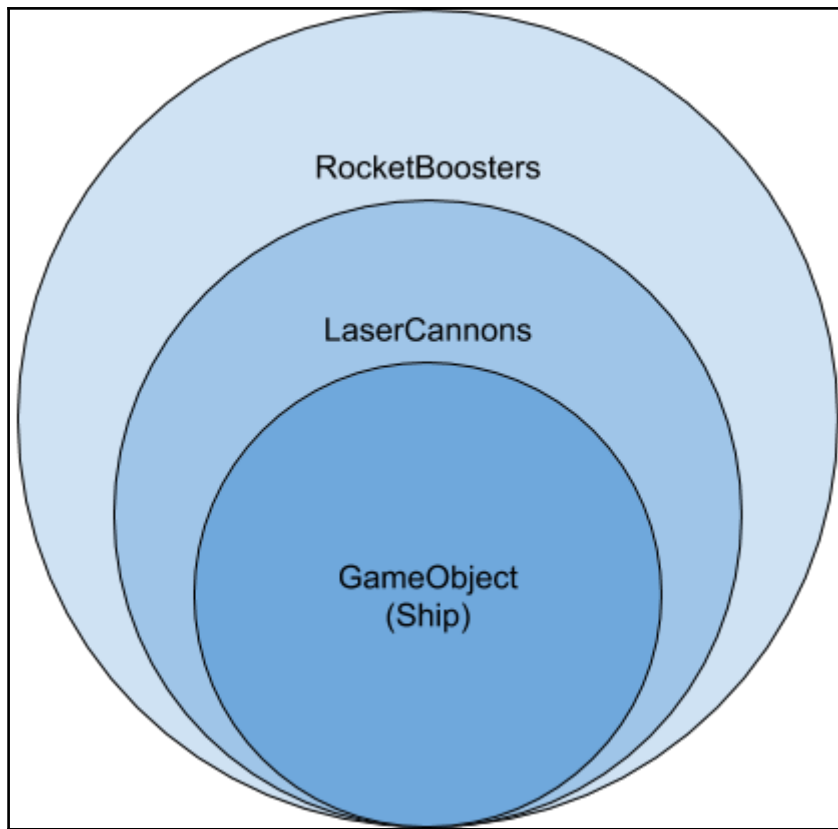
Figure 3.7 - The layering effects of the Decorator pattern
