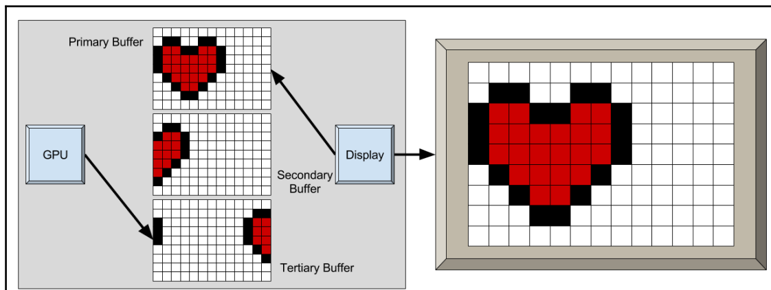
Figure 11.13 - Drawing to the tertiary buffer before the V-Blank
