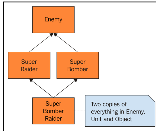
Figure 3.5 - Example of the Diamond of Death
