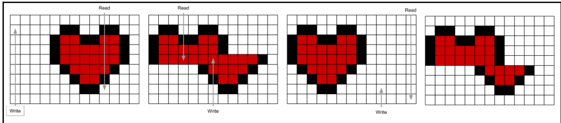
Figure 11.8 - Example of tearing in the framebuffer
