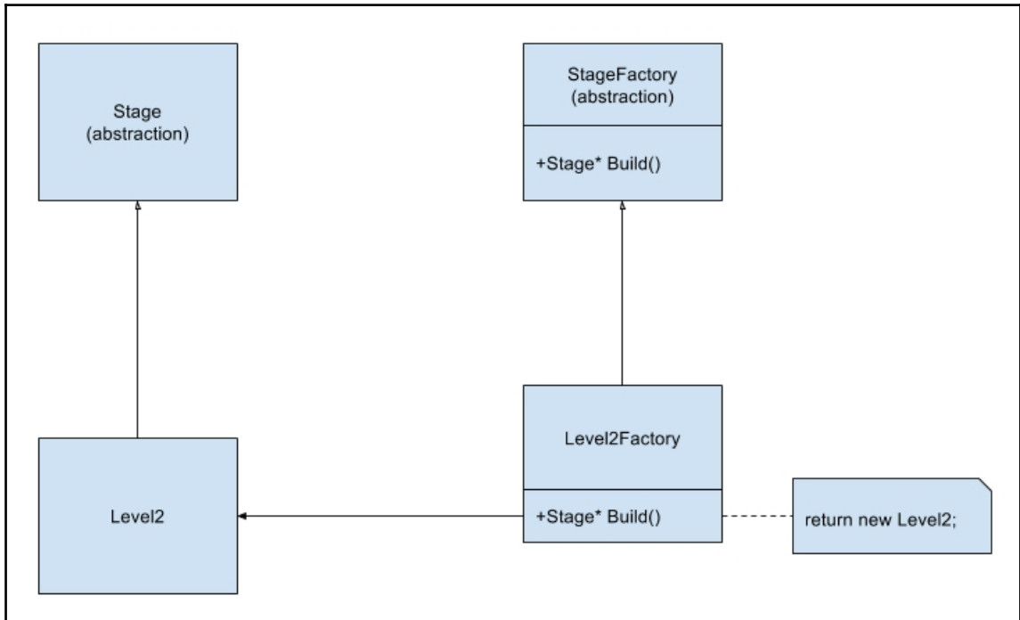
Creating a Stage Factory
