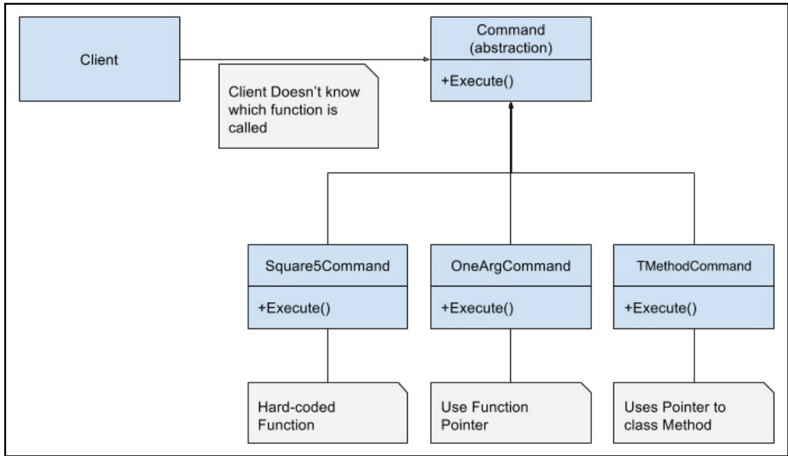
Figure 8.3 - The command hierarchy
