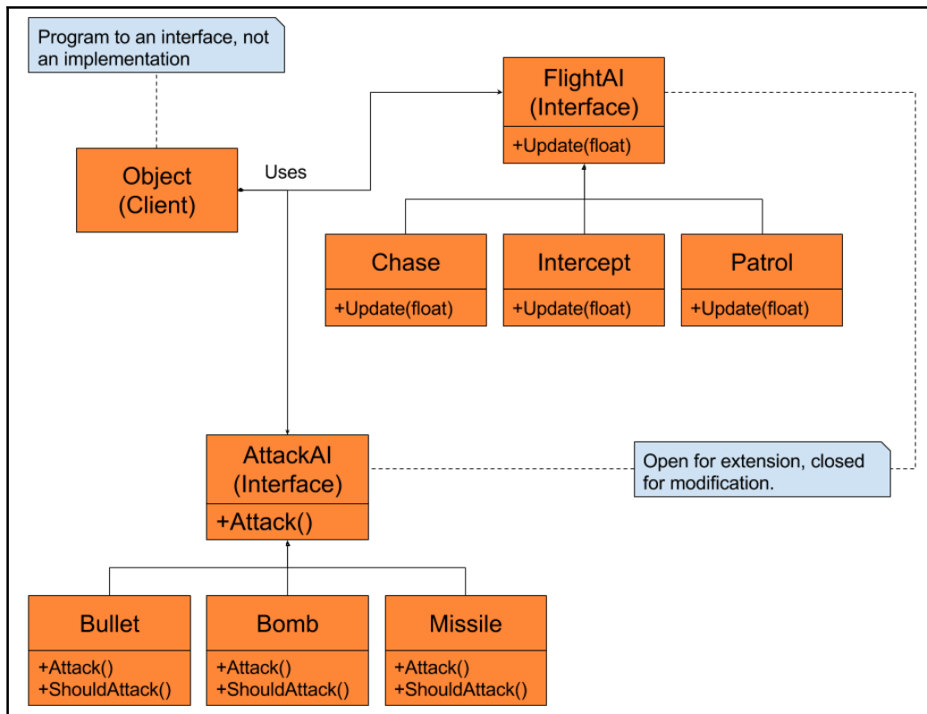
Figure 3.6 - Example of our Object using the Strategy pattern
